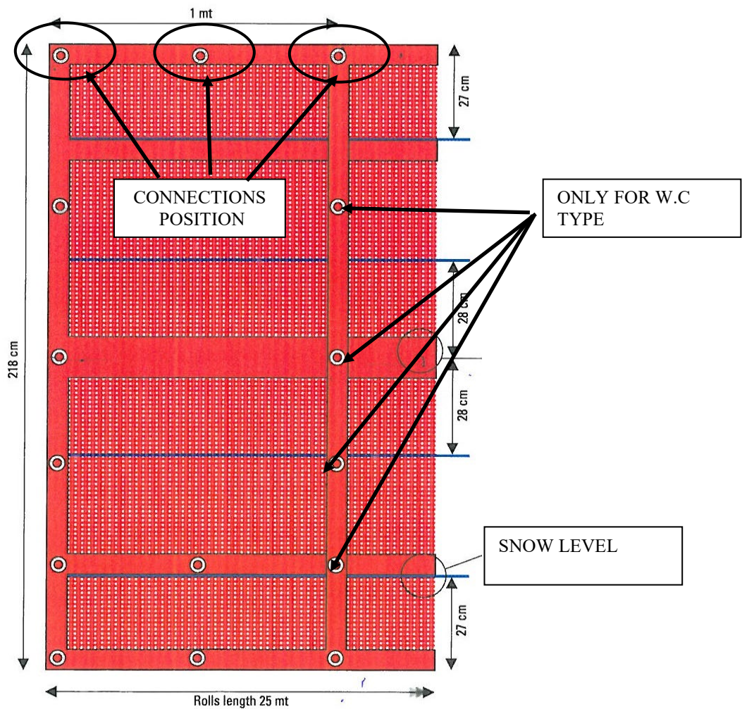
Step 2 Attaching connection system to nets
