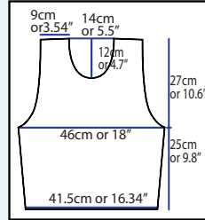
FIS Mens Cross Country LBN200M 3/4 inch flat hem on bottom No Elastic
