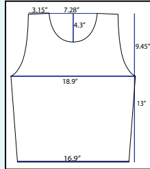
FIS Mens Alpine Bib LBA 100M No Bias Double overlock stitch neck & arm holes Flat bottom hem with 3/4 inch Elastic
